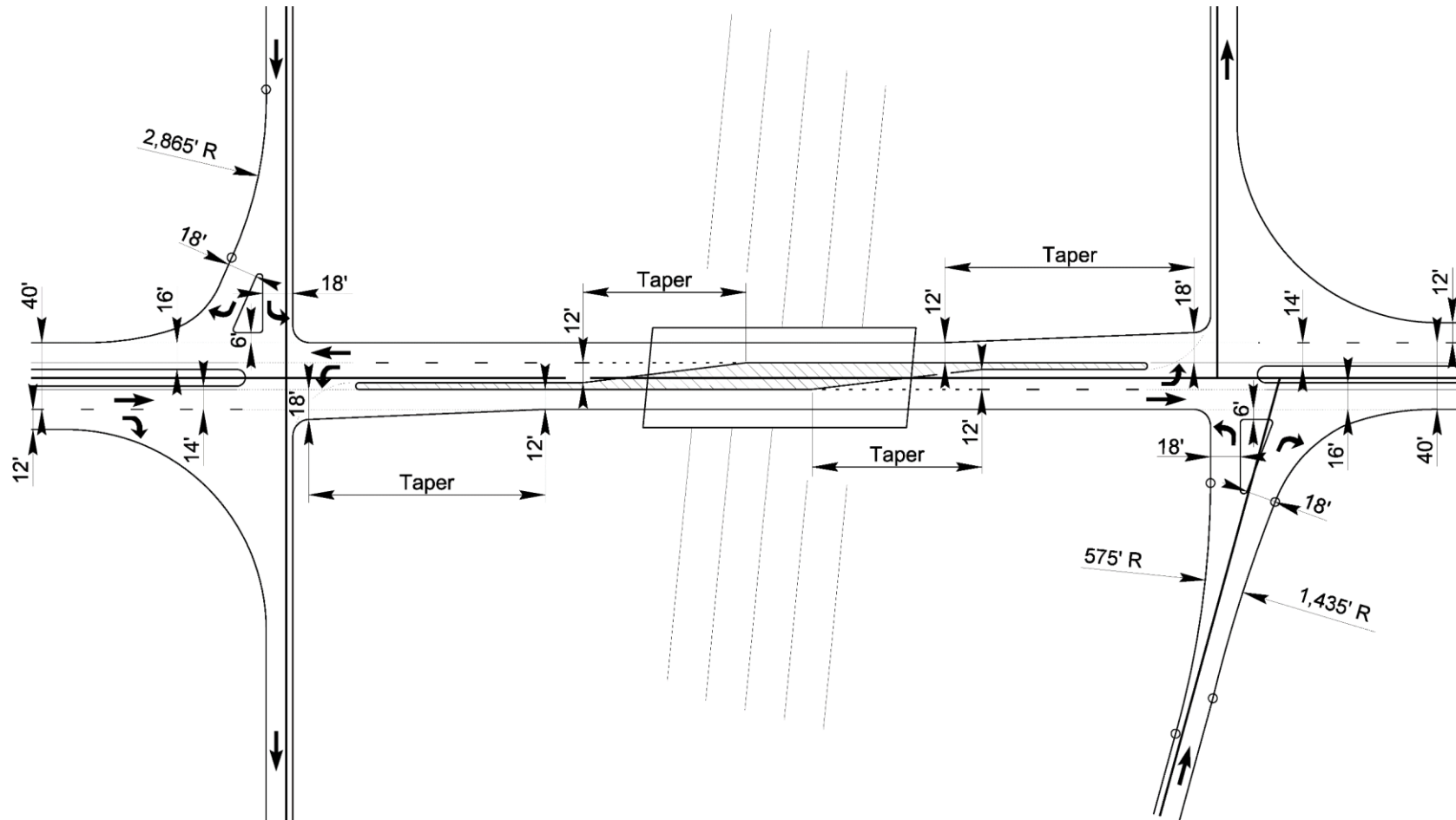
Figure 9-8 Ramp Terminal Design
