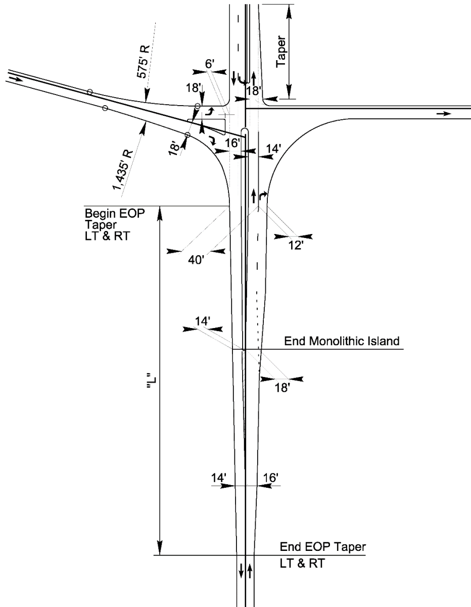
Figure 9-7 -Y- Line Transition at Ramp Terminal for Three-Lane -Y- Line Section
