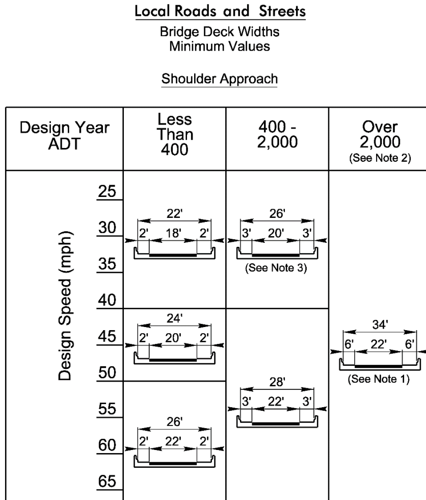
Figure 5-8 Local Roads and Streets Bridge Deck Widths
